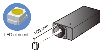
System for measuring average luminous intensity (0.01 sr)
