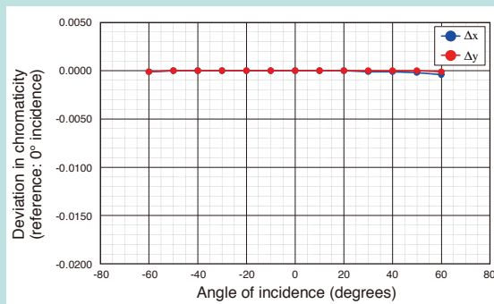
Figure 5. Incident Angle Dependence
