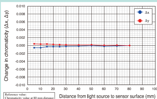
Figure 6. Effect of Measurement Distance (with \phi 6.3\text{ mm} Light Source)
