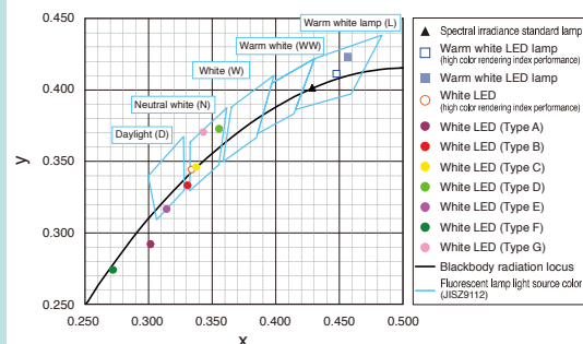
Figure 3. Chromaticity Values (Chromaticity Measurement Results for 10 Types of White LED)
