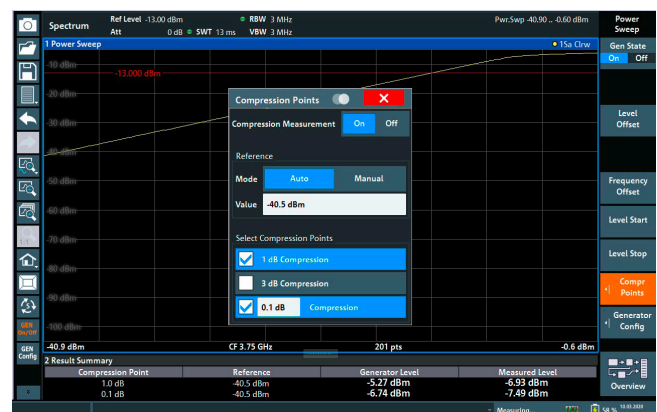
Measurement of 1 dB and 0.1 dB compression points
