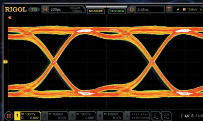
Use the 600 MHz bandwidth and 2 GHz bandwidth model respectively to perform eye measurement on the 1 Gb/s signal.
