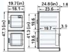
MCU-301A 11 cf (2-door type)
