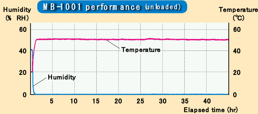
Fan-equipped baking unit for MB-1001
