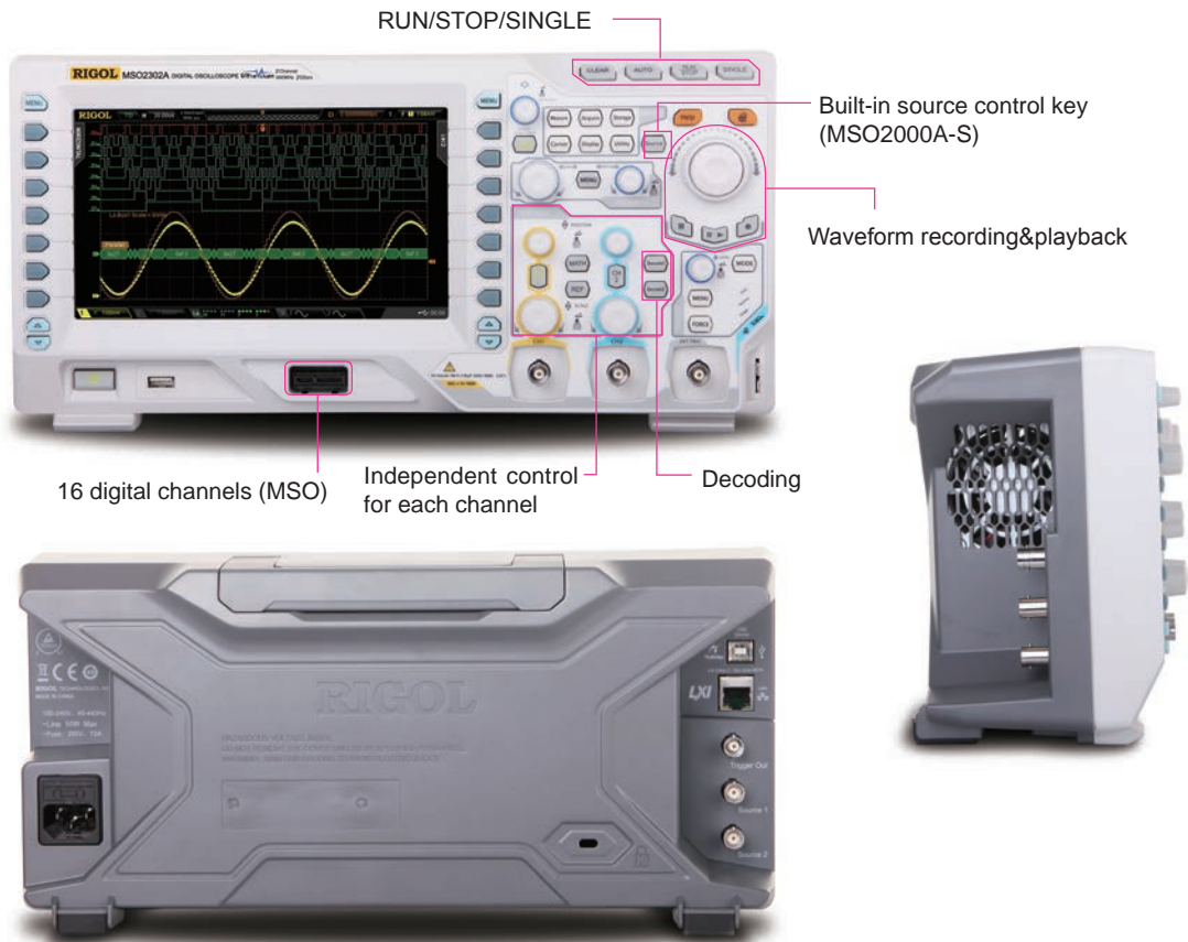
Product Dimensions: WidthxHeightxDepth = 361.6 mmx179.6 mmx130.8 mm Weight: 3.9 kg±0.5 kg (Without Package)
