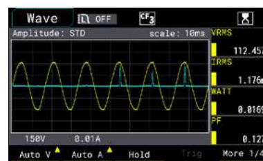
Waveform Display of Voltage and Current
