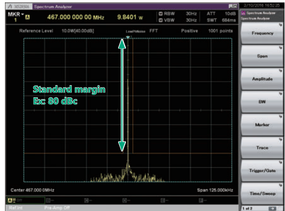
Spurious Emissions (out-of-band) Measurement Example
