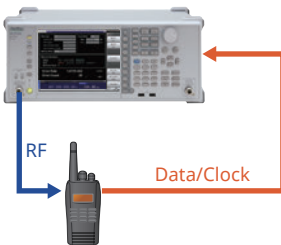
Rx Sensitivity Test Setup
