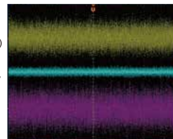
Top: Conventional model (Bandwidth is fixed at 26 MHz) Middle: Conventional model 1 MHz LPF passed separately Bottom: WF1983 (Bandwidth : 1MHz)
