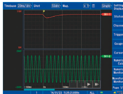
• Example of instrument recording the instantaneous waveform and RMS level waveform during a momentary outage of an AC power supply (using the MR8905)
