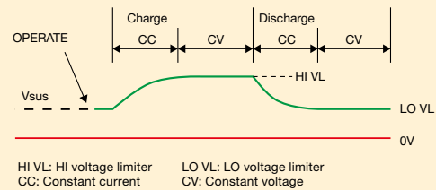
Battery Charge Waveform
