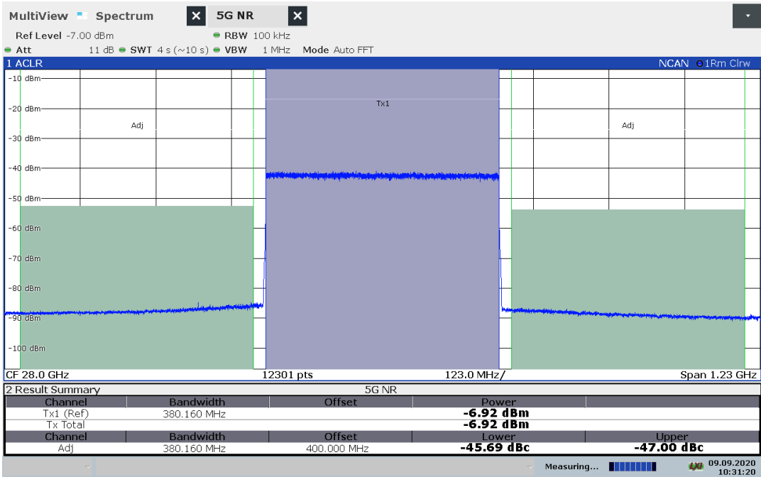
Measured ACPR at 28 GHz for a 5G NR test model NR-FR2-TM3.1; TDD 400 MHz bandwidth, -120 kHz SCS
